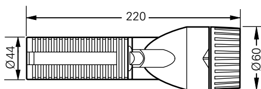
Dimension drawing Stabceag 0
