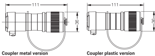
Coupler metal version
